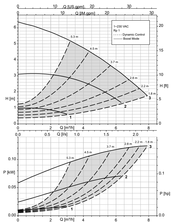
Calio Pro 25-60 Open-loop Control, Dynamic Control
