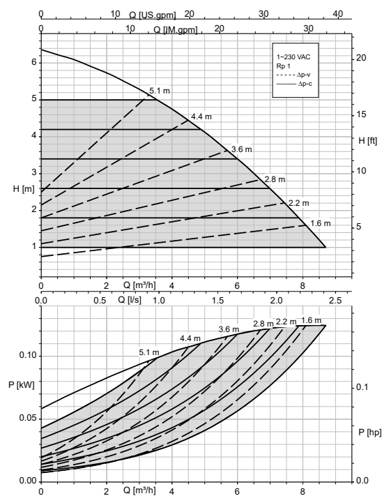
Calio Pro 25-60 \Delta p_v , \Delta p_c
