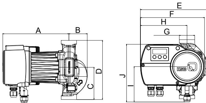
Fig. 3: Screw-ended pump set
